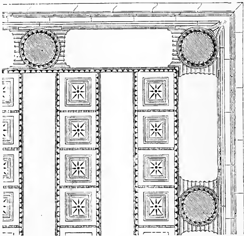
FIG. 89—PLAN OF THE PORTICO—LOOKING UP.
